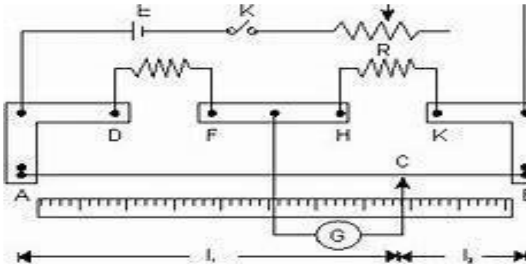
The Meter Bridge Fig. 14.4
