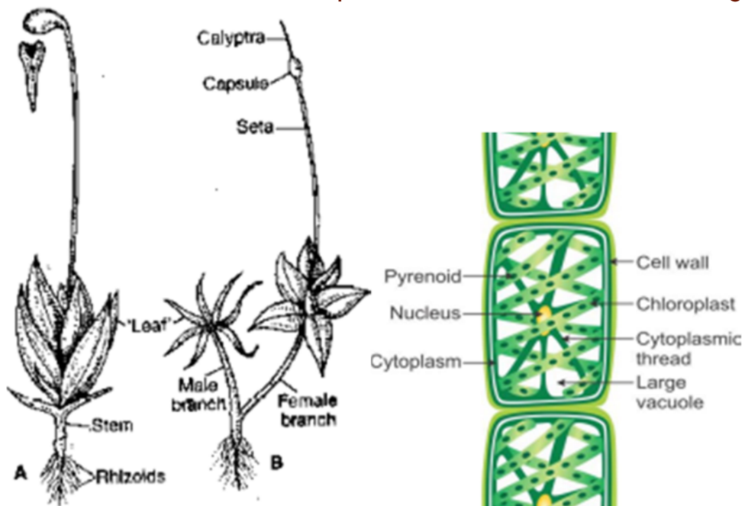
spiogyra funaria
